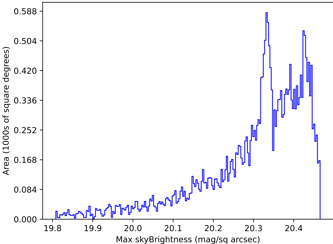
early_u_fpextra2.0_v3.4_10yrs All sky i band: Max skyBrightness
