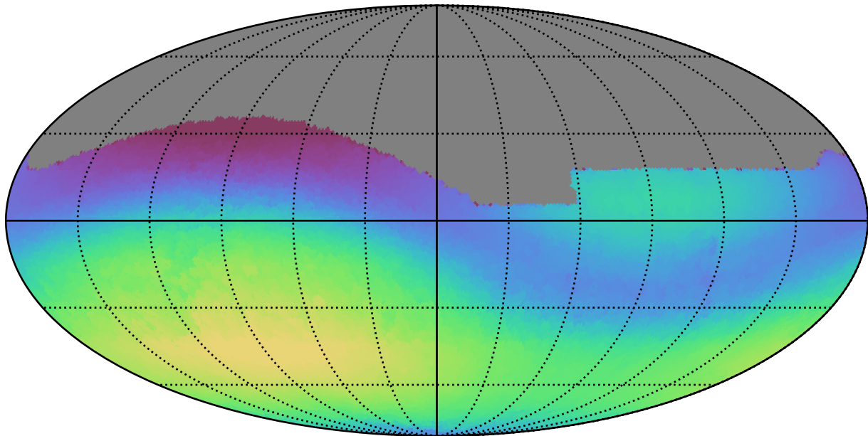
early_u_fpextra2.0_v3.4_10yrs All sky g band: Max skyBrightness
