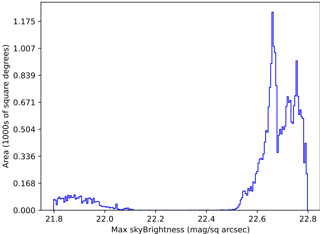
early_u_fpextra2.0_v3.4_10yrs All sky all bands: Max skyBrightness
