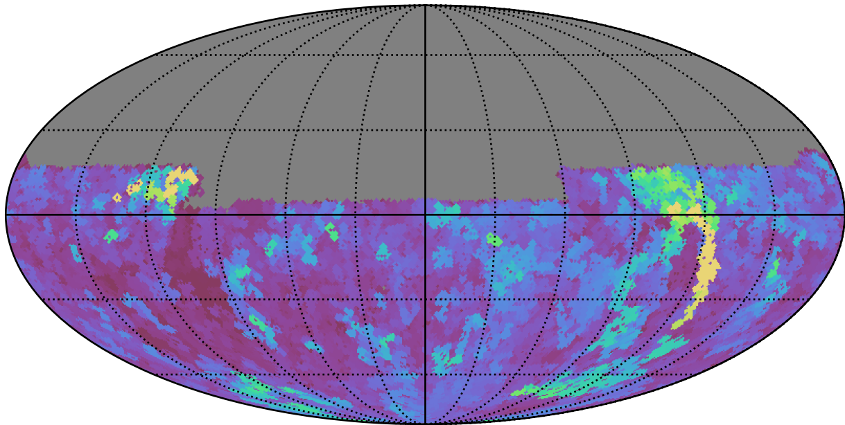
early_u_fpextra2.0_v3.4_10yrs Yr 1 u band: Max seeingGeom
