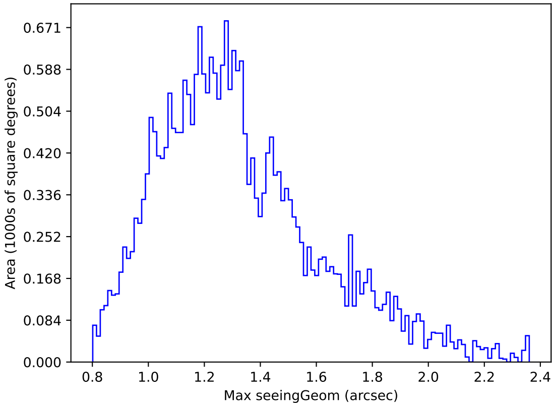
early_u_fpextra2.0_v3.4_10yrs Yr 1 r band: Max seeingGeom
