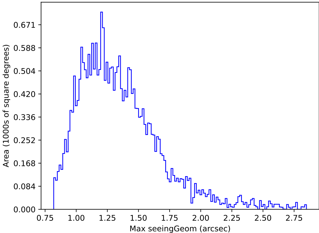
early_u_fpextra2.0_v3.4_10yrs Yr 1 i band: Max seeingGeom
