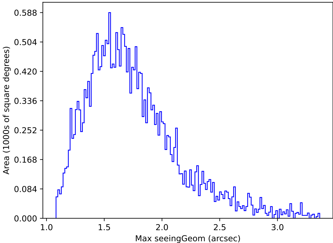
early_u_fpextra2.0_v3.4_10yrs Yr 1 all bands: Max seeingGeom
