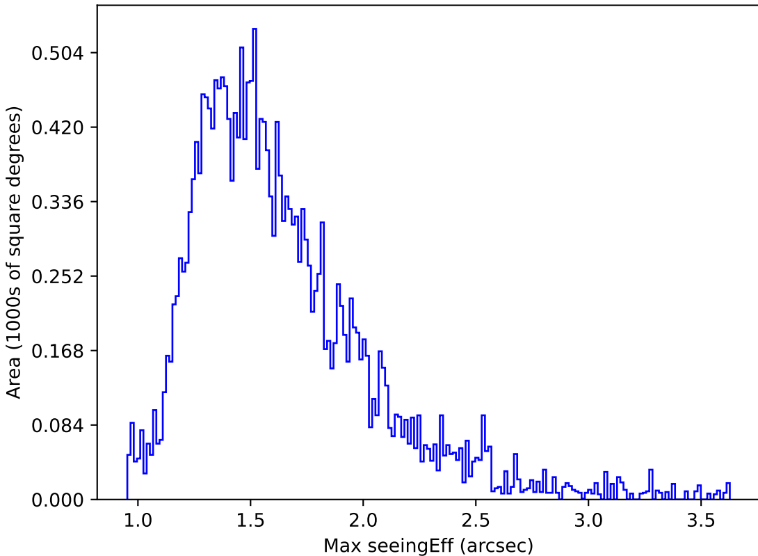
early_u_fpextra2.0_v3.4_10yrs Yr 1 u band: Max seeingEff
