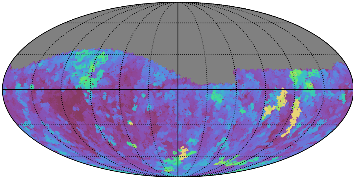
early_u_fpextra2.0_v3.4_10yrs Yr 1 g band: Max seeingEff
