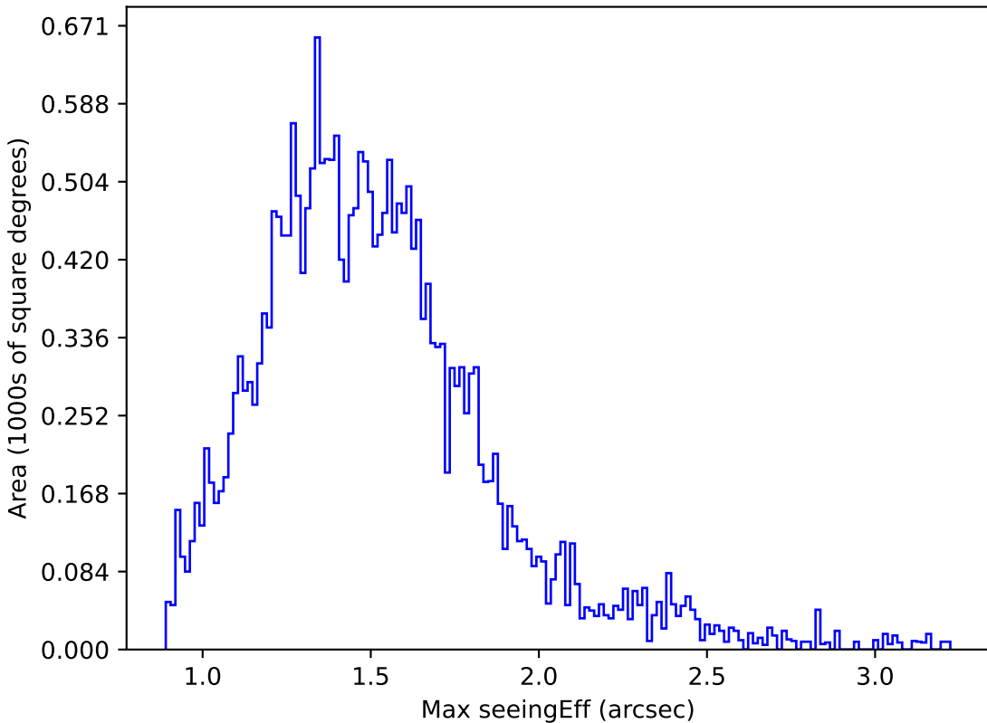
early_u_fpextra2.0_v3.4_10yrs Yr 1 g band: Max seeingEff
