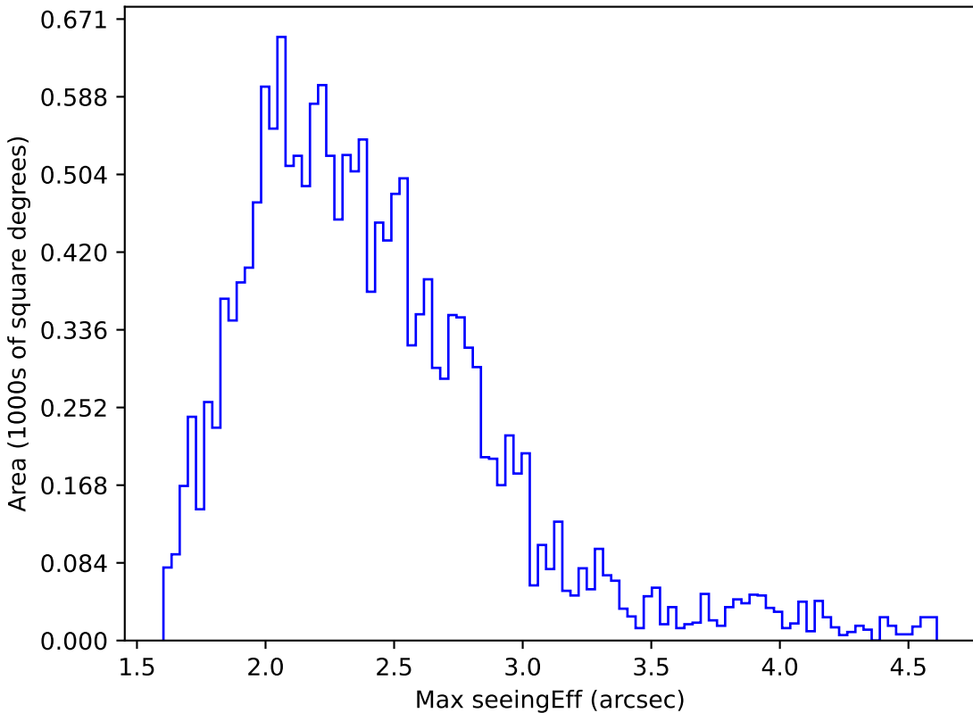
early_u_fpextra2.0_v3.4_10yrs WFD y band: Max seeingEff
