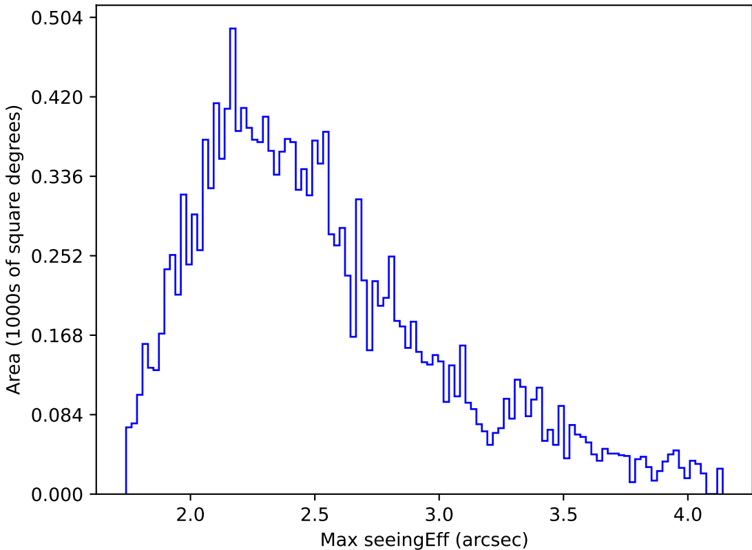
early_u_fpextra2.0_v3.4_10yrs WFD u band: Max seeingEff
