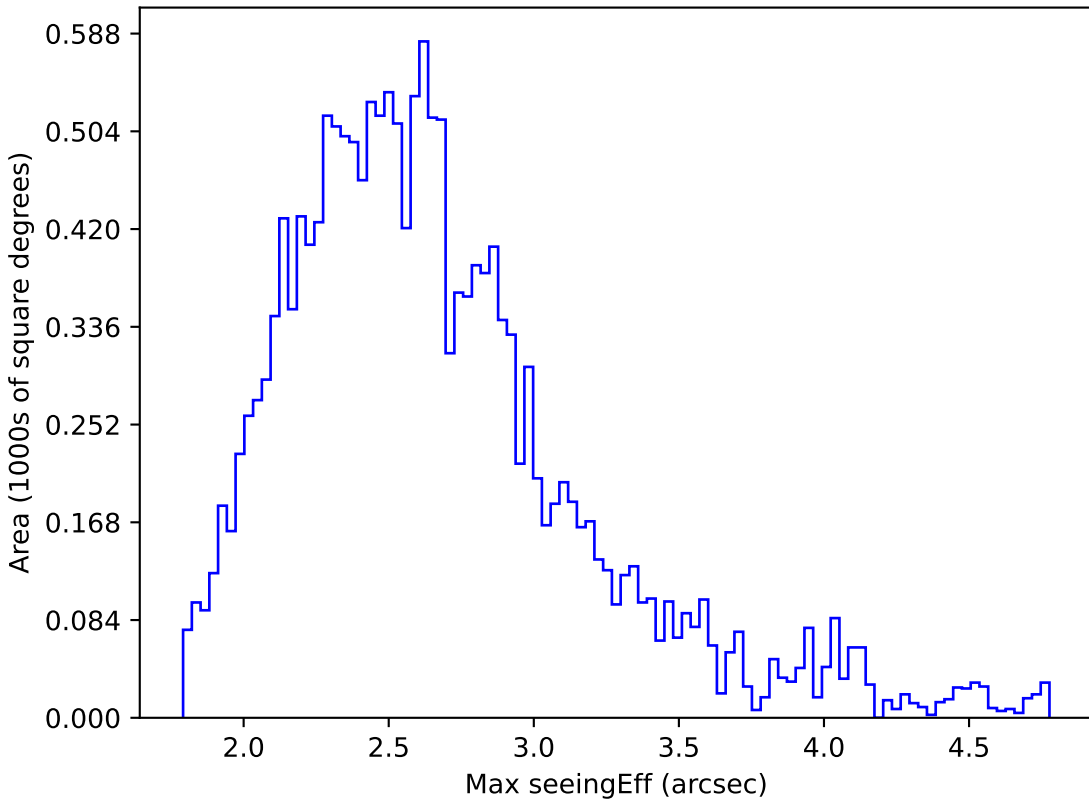
early_u_fpextra2.0_v3.4_10yrs WFD r band: Max seeingEff
