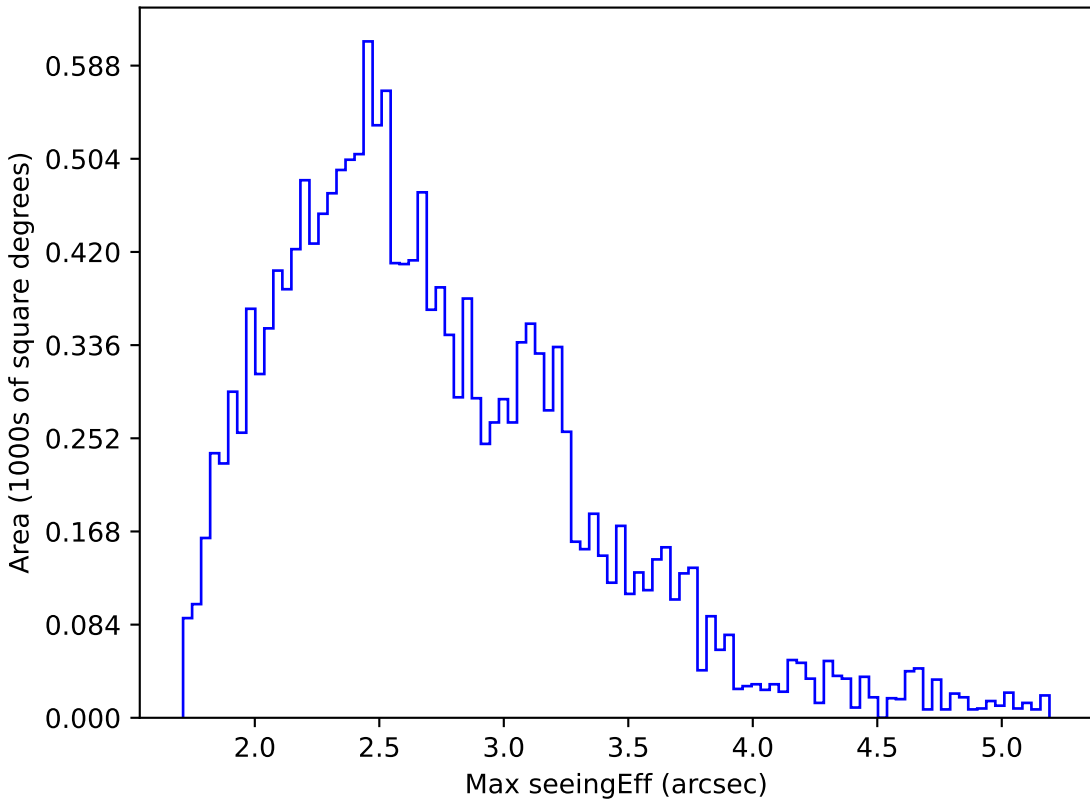
early_u_fpextra2.0_v3.4_10yrs WFD i band: Max seeingEff
