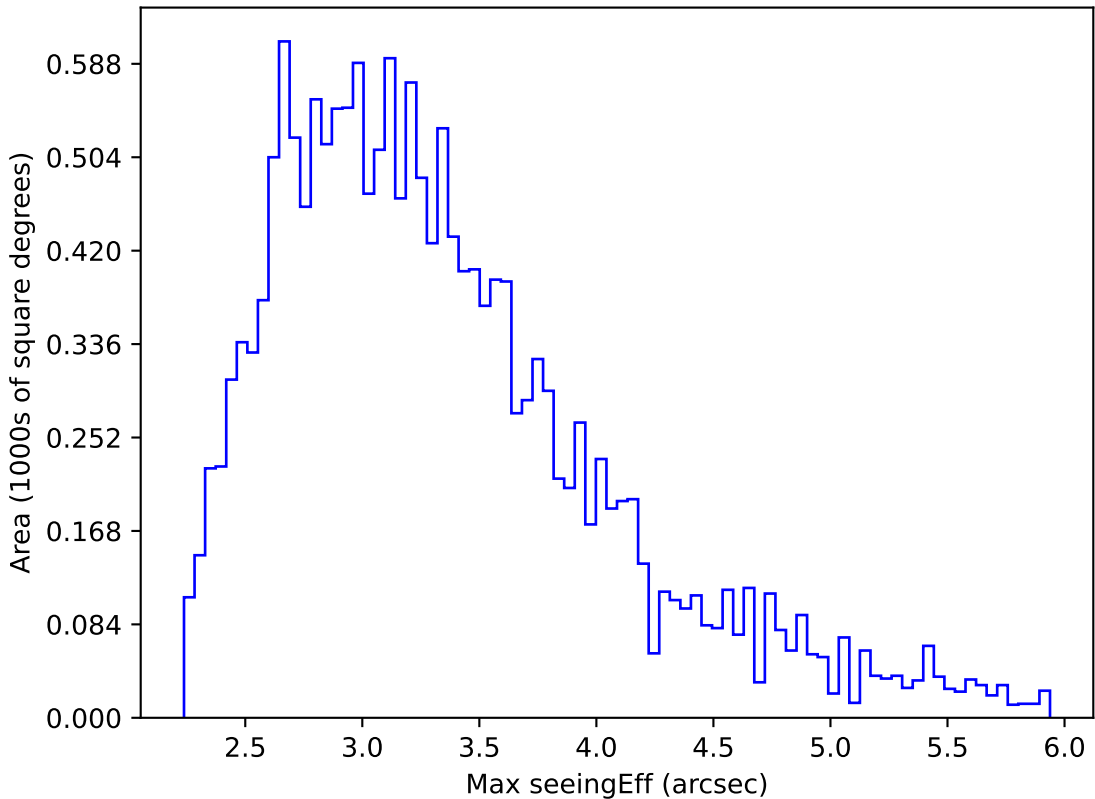
early_u_fpextra2.0_v3.4_10yrs WFD all bands: Max seeingEff
