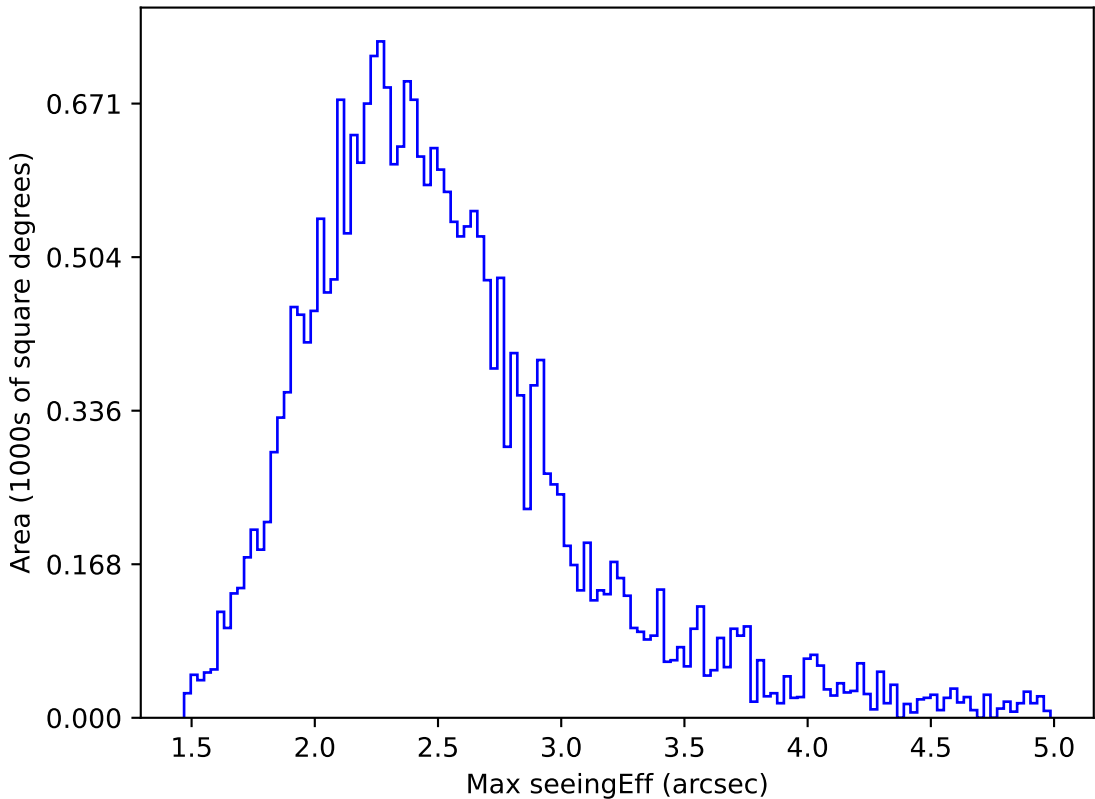
early_u_fpextra2.0_v3.4_10yrs All sky z band: Max seeingEff
