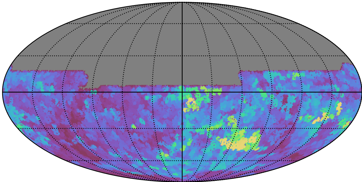
early_u_fpextra2.0_v3.4_10yrs All sky y band: Max seeingEff
