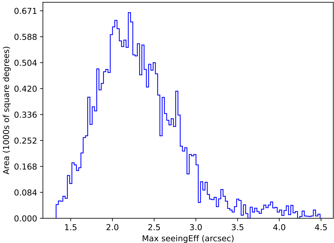
early_u_fpextra2.0_v3.4_10yrs All sky y band: Max seeingEff
