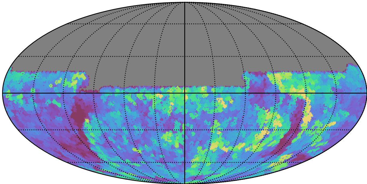
early_u_fpextra2.0_v3.4_10yrs All sky u band: Max seeingEff
