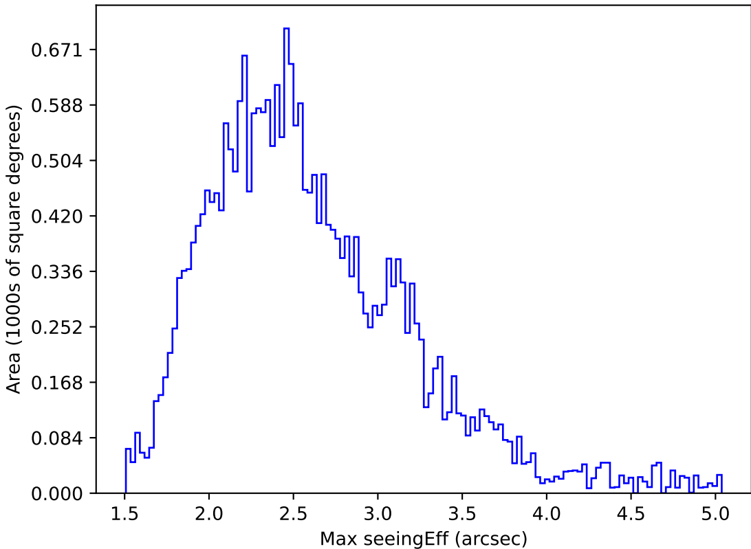
early_u_fpextra2.0_v3.4_10yrs All sky i band: Max seeingEff
