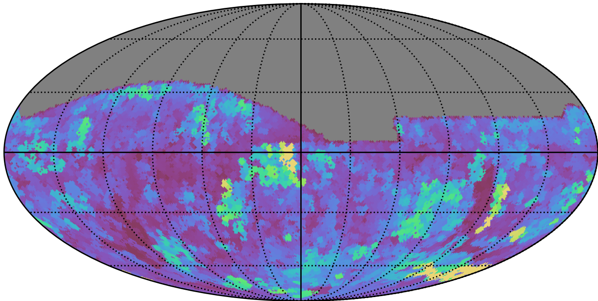
early_u_fpextra2.0_v3.4_10yrs All sky g band: Max seeingEff
