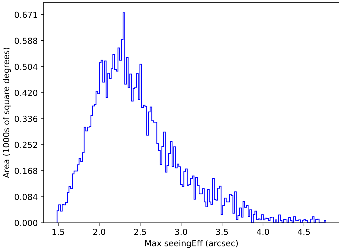
early_u_fpextra2.0_v3.4_10yrs All sky g band: Max seeingEff
