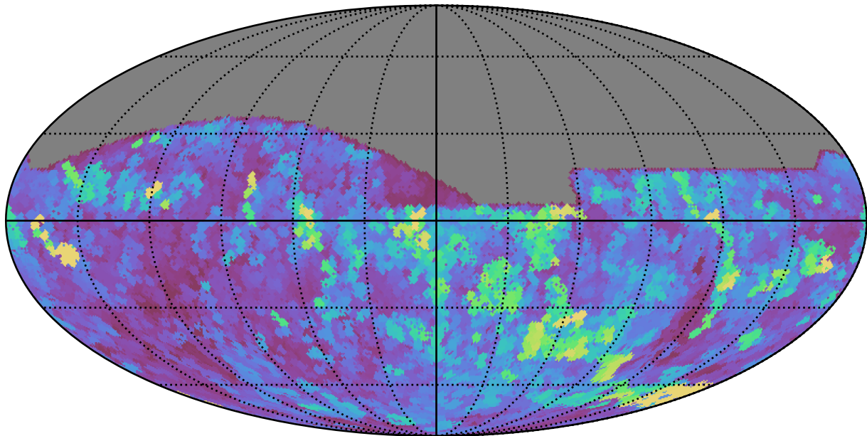
early_u_fpextra2.0_v3.4_10yrs All sky all bands: Max seeingEff
