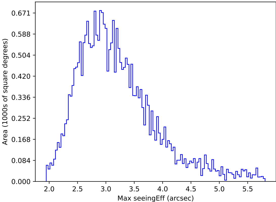
early_u_fpxextra2.0_v3.4_10yrs All sky all bands: Max seeingEff
