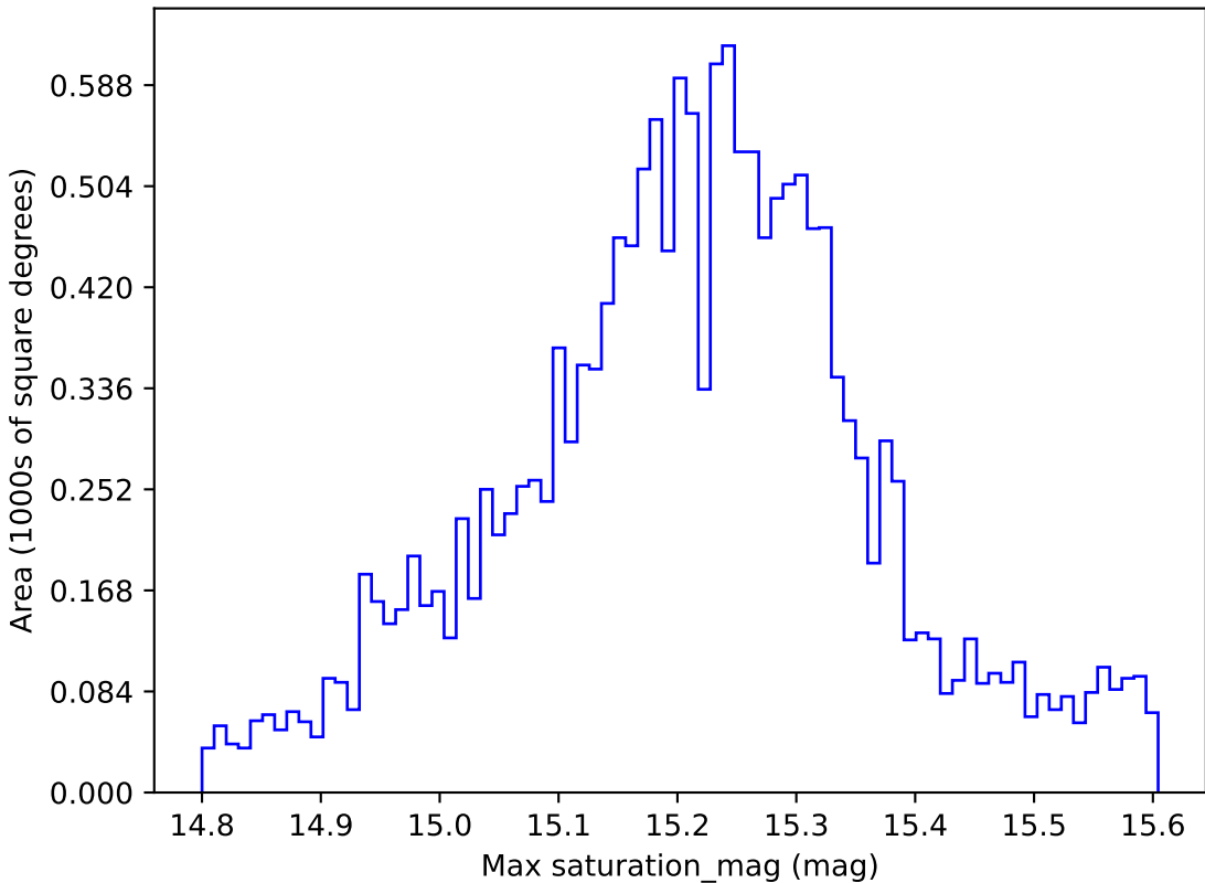
early_u_fpextra2.0_v3.4_10yrs WFD z band: Max saturation_mag
