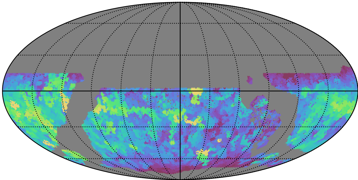
early_u_fpextra2.0_v3.4_10yrs WFD u band: Max saturation_mag
