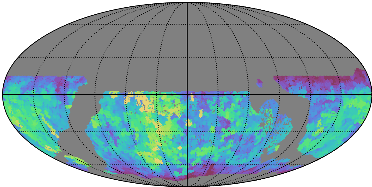
early_u_fpextra2.0_v3.4_10yrs WFD g band: Max saturation_mag
