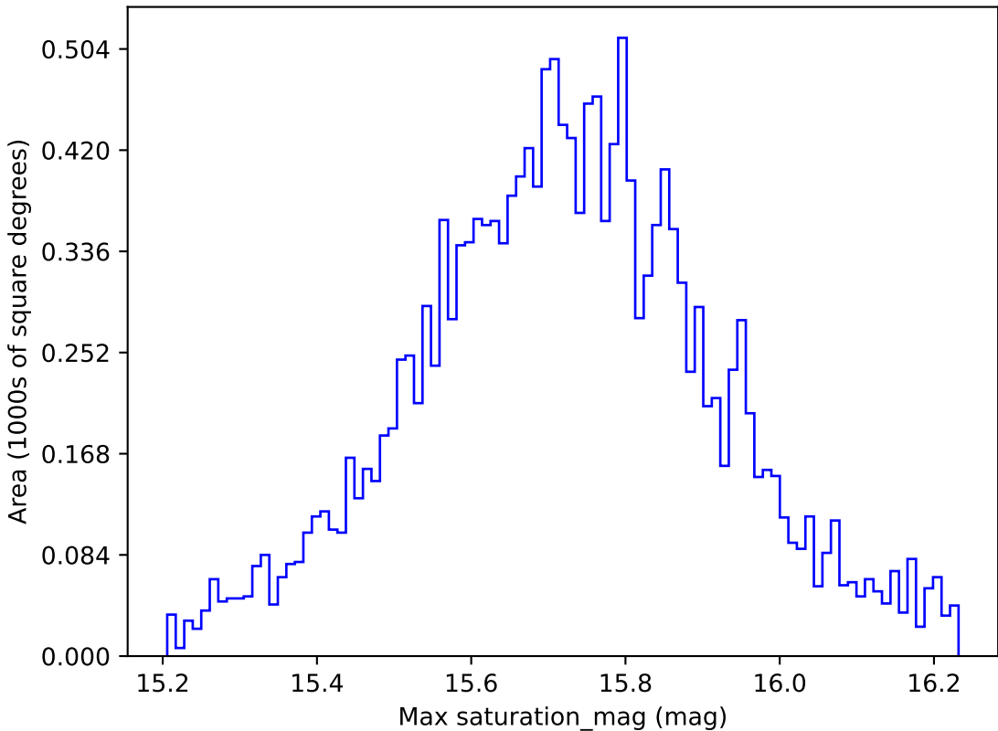
early_u_fpextra2.0_v3.4_10yrs WFD g band: Max saturation_mag
