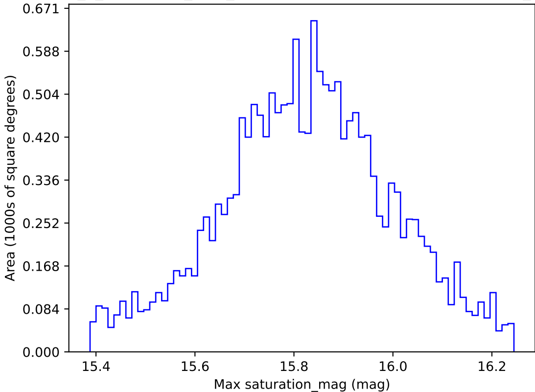
early_u_fpextra2.0_v3.4_10yrs WFD all bands: Max saturation_mag
