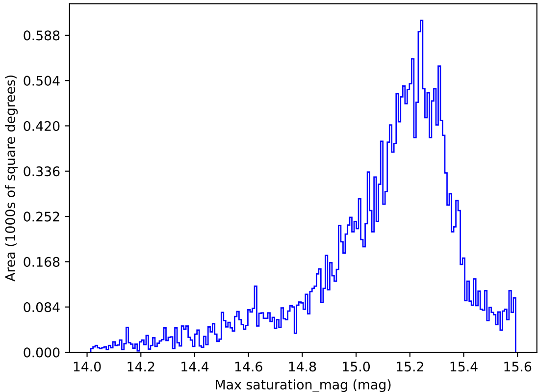
early_u_fpextra2.0_v3.4_10yrs All sky z band: Max saturation_mag
