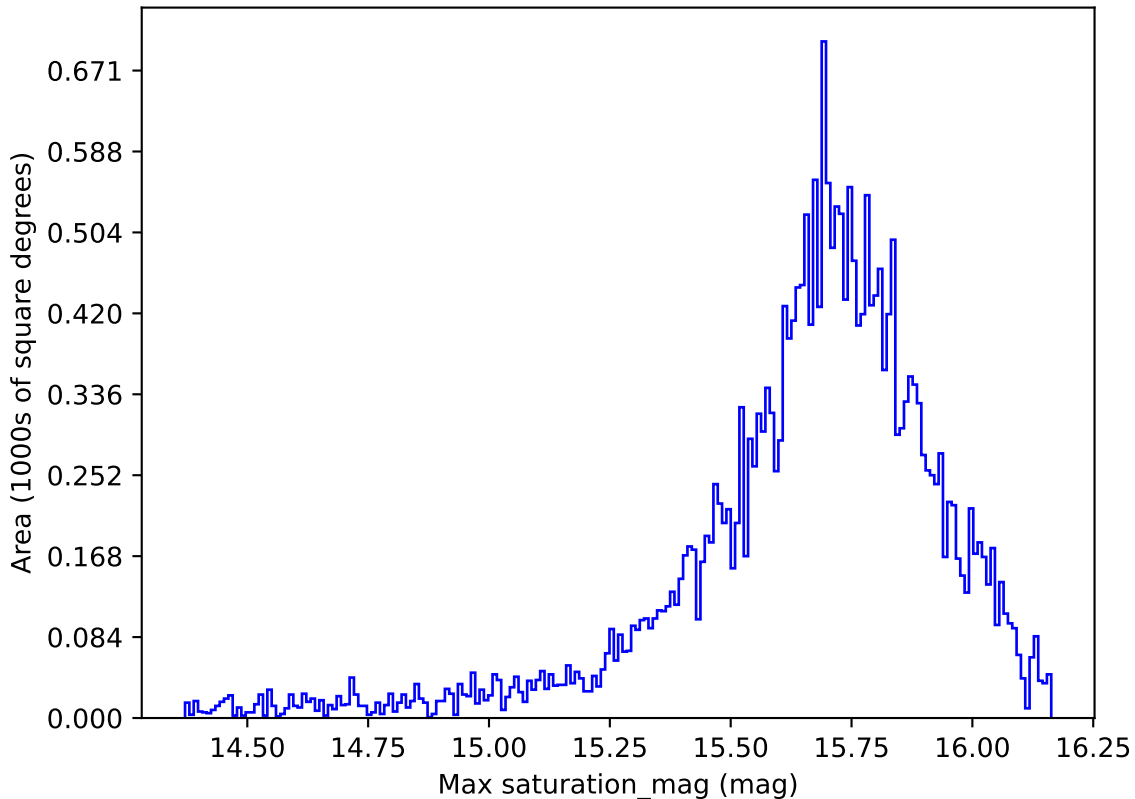
early_u_fpextra2.0_v3.4_10yrs All sky r band: Max saturation_mag
