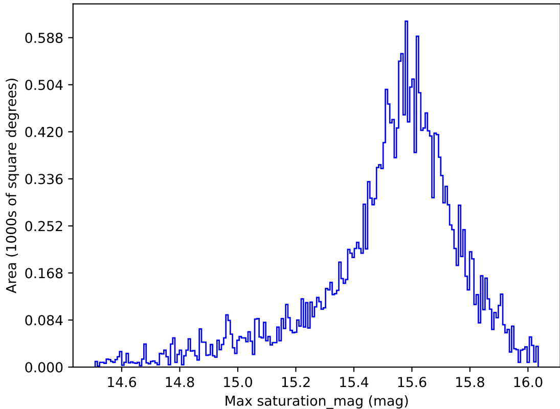
early_u_fpextra2.0_v3.4_10yrs All sky i band: Max saturation_mag
