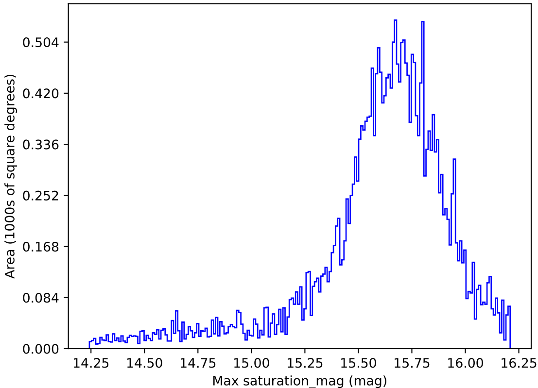
early_u_fpextra2.0_v3.4_10yrs All sky g band: Max saturation_mag
