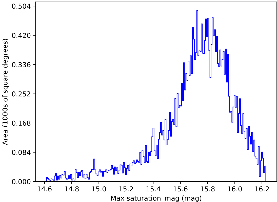
early_u_fpextra2.0_v3.4_10yrs All sky all bands: Max saturation_mag
