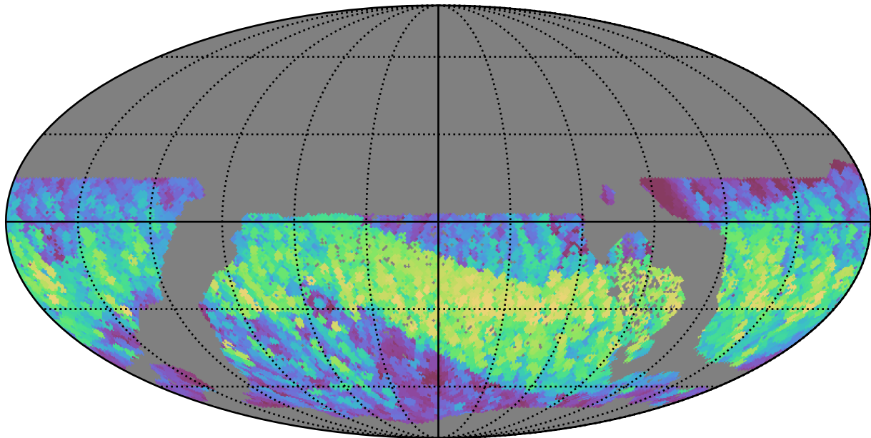
early_u_fpextra2.0_v3.4_10yrs WFD z band: Max normairmass
