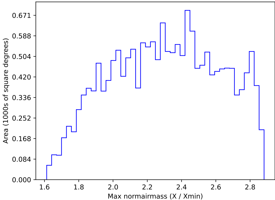
early_u_fpextra2.0_v3.4_10yrs WFD z band: Max normairmass
