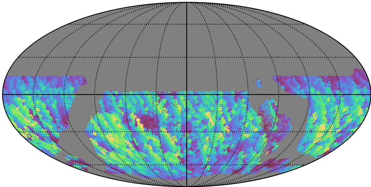
early_u_fpextra2.0_v3.4_10yrs WFD y band: Max normairmass
