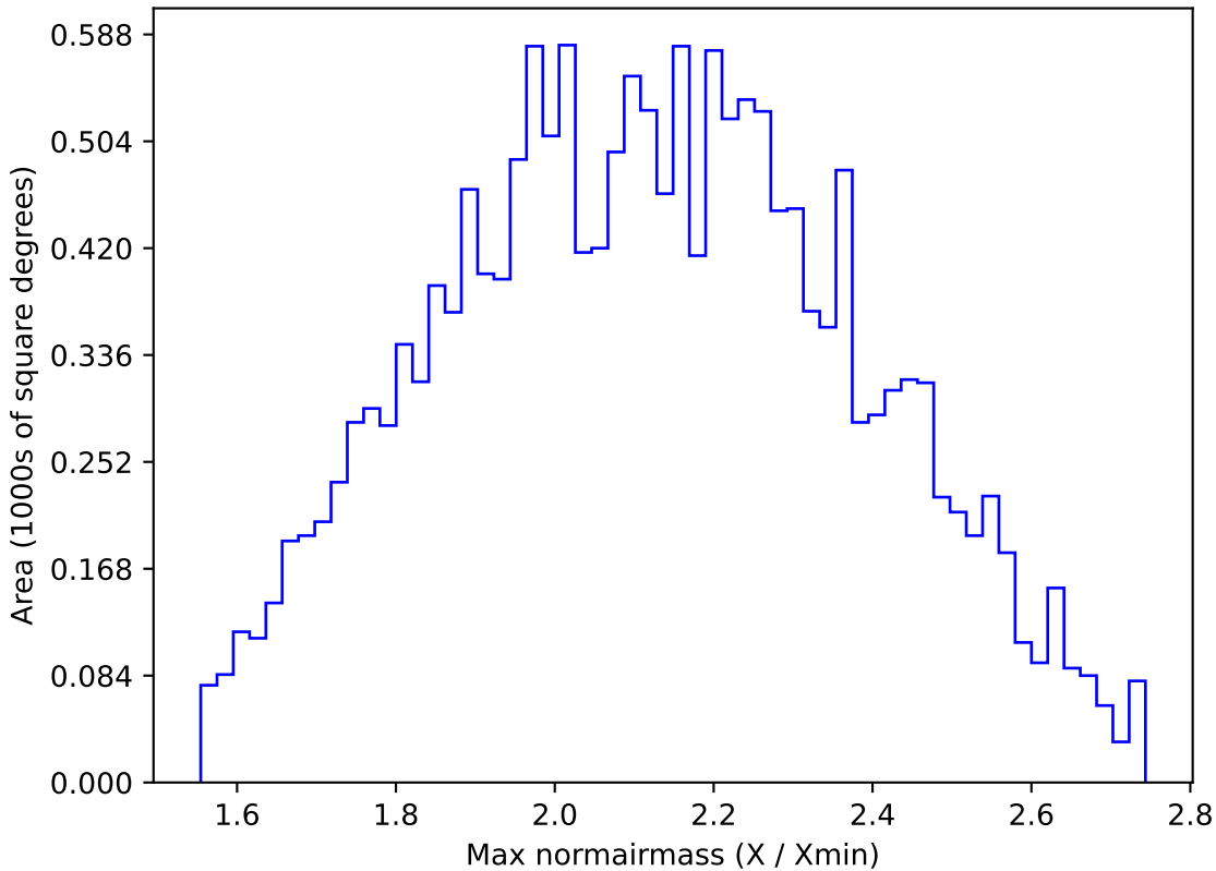
early_u_fpextra2.0_v3.4_10yrs WFD y band: Max normairmass
