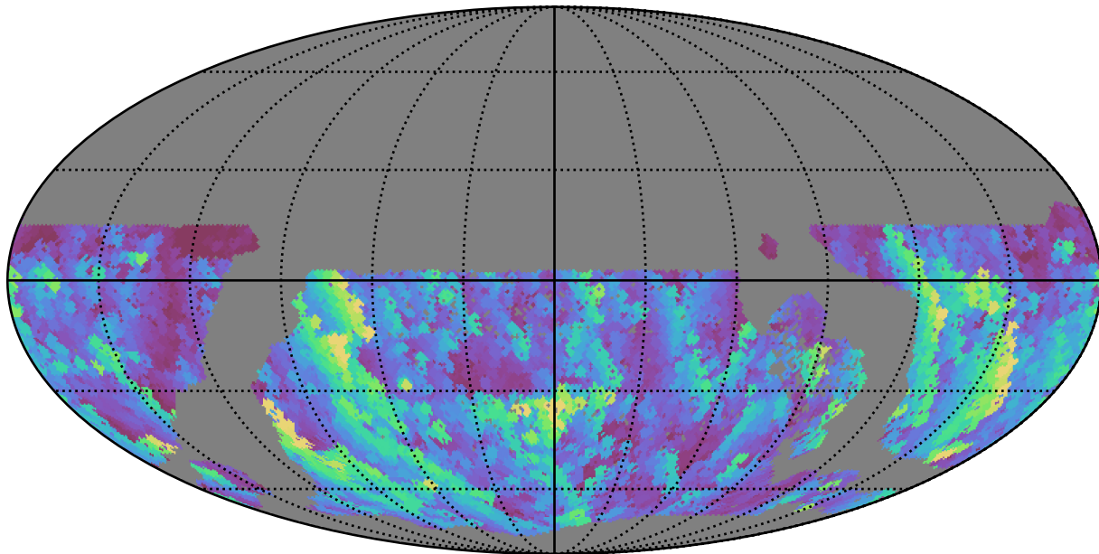
early_u_fpextra2.0_v3.4_10yrs WFD u band: Max normairmass
