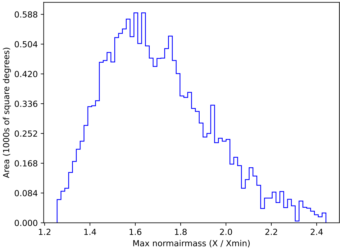
early_u_fpextra2.0_v3.4_10yrs WFD u band: Max normairmass
