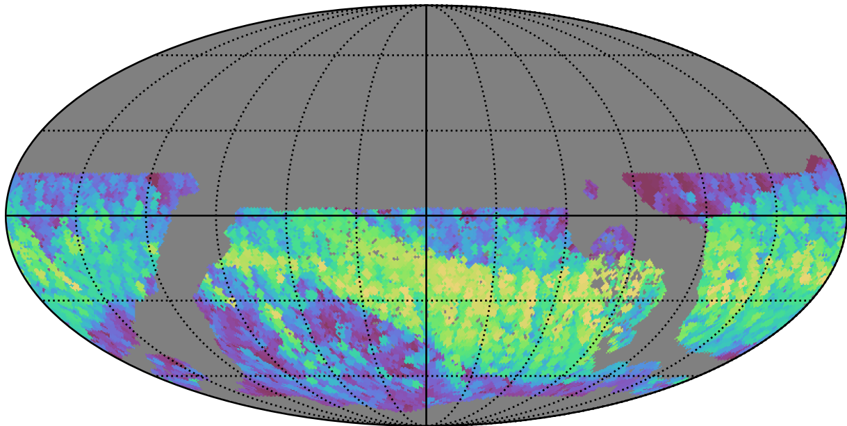
early_u_fpextra2.0_v3.4_10yrs WFD i band: Max normairmass
