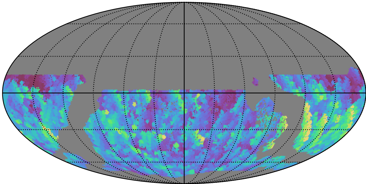
early_u_fpextra2.0_v3.4_10yrs WFD g band: Max normairmass
