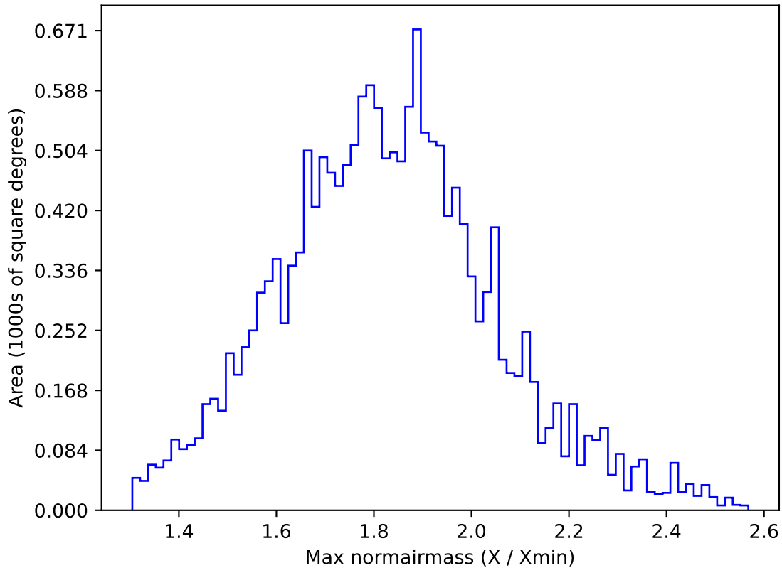
early_u_fpextra2.0_v3.4_10yrs WFD g band: Max normairmass
