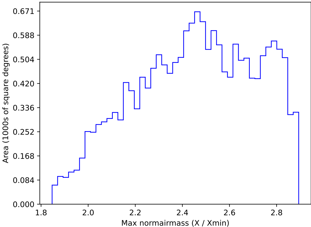
early_u_fpextra2.0_v3.4_10yrs WFD all bands: Max normairmass
