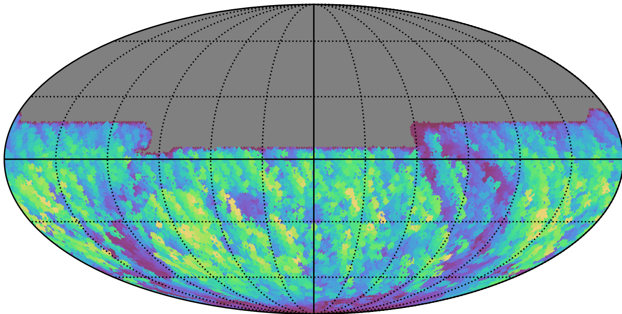
early_u_fpextra2.0_v3.4_10yrs All sky y band: Max normairmass
