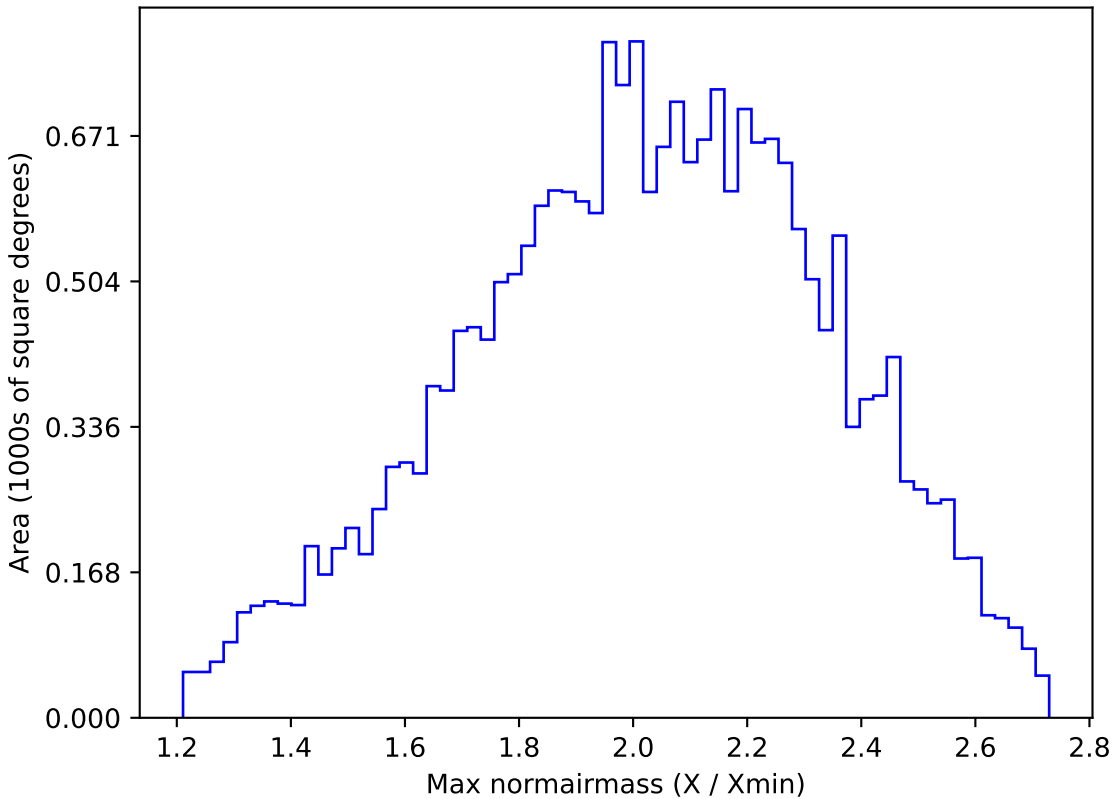
early_u_fpextra2.0_v3.4_10yrs All sky y band: Max normairmass
