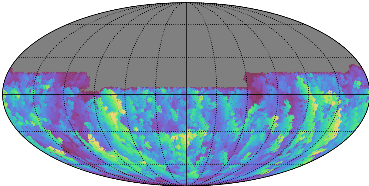
early_u_fpextra2.0_v3.4_10yrs All sky u band: Max normairmass
