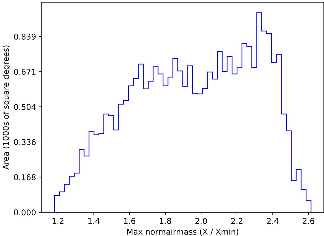
early_u_fpextra2.0_v3.4_10yrs All sky r band: Max normairmass
