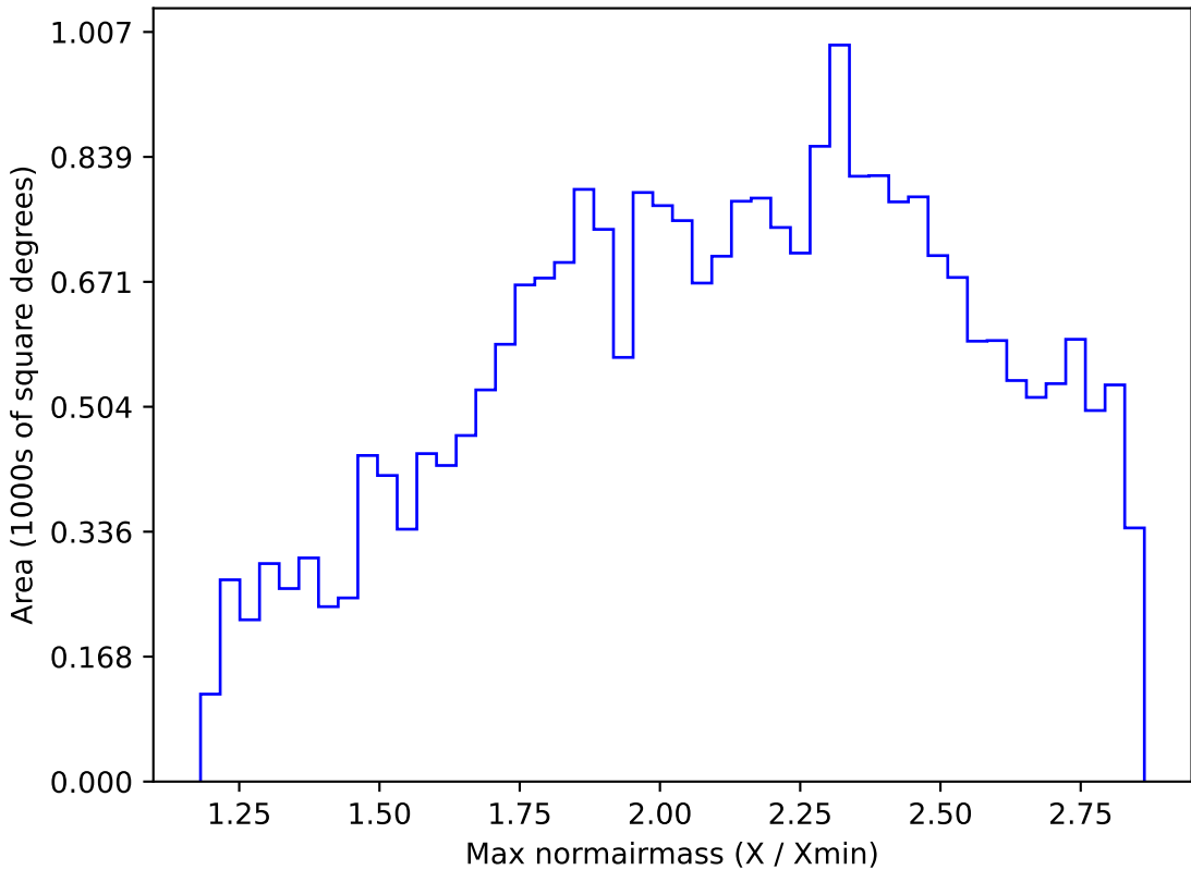
early_u_fpextra2.0_v3.4_10yrs All sky i band: Max normairmass
