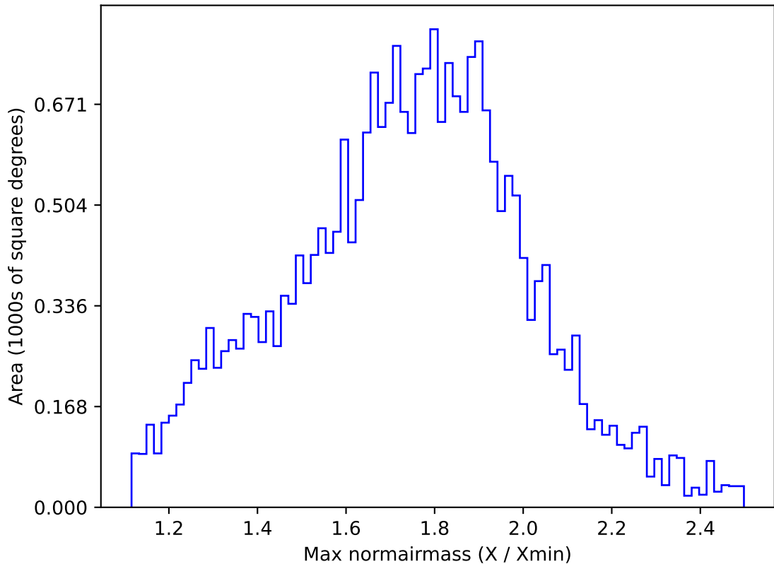
early_u_fpextra2.0_v3.4_10yrs All sky g band: Max normairmass
